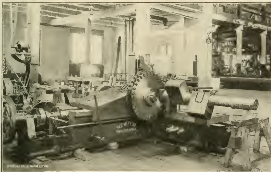
NEWTON COLD METAL CUTTING OFF MACHINE WITH TAYLOR-NEUBOLD SAW.
